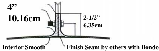
Flange for Bolt
